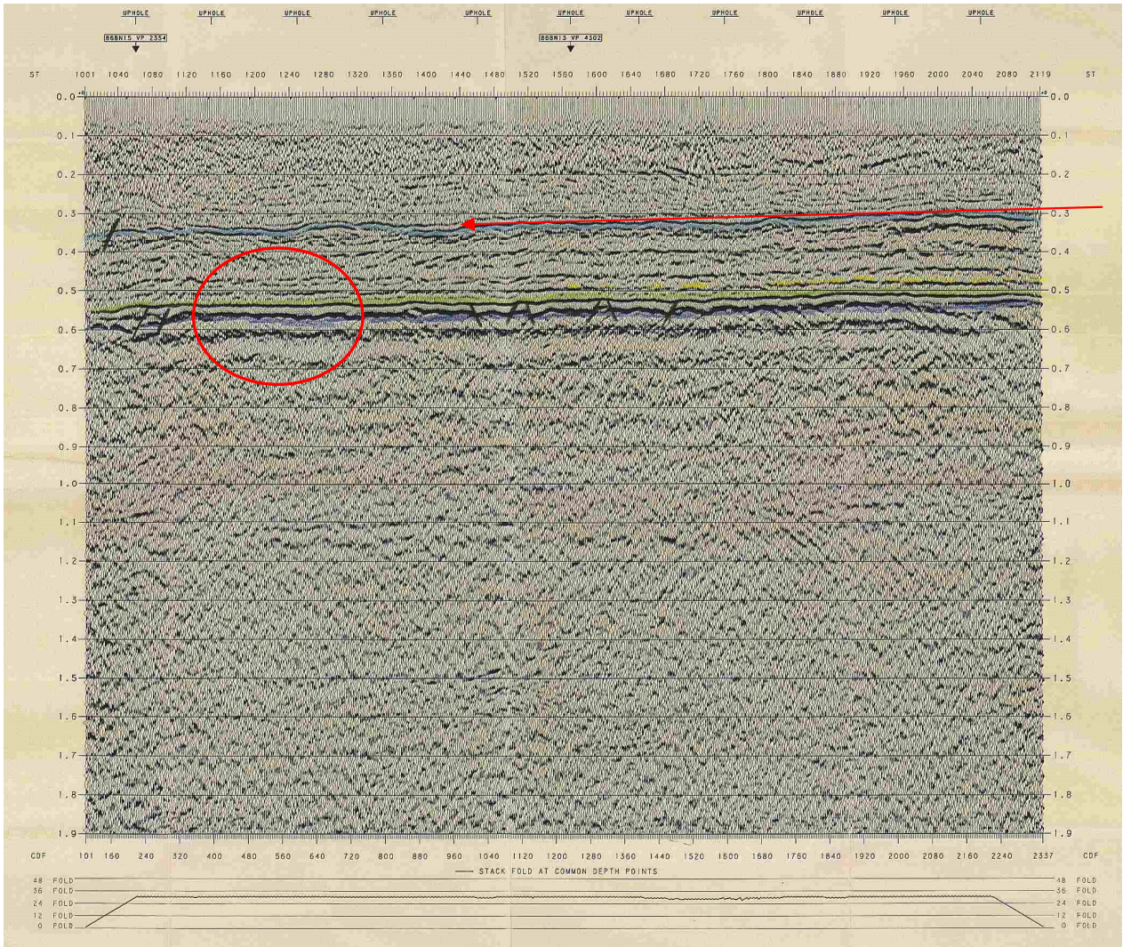
Figure 13: Line 86BN16 with Comalco interpretation.
