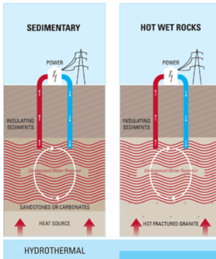
Figure 3: Simplified diagram of Hot Sedimentary Rock systems
