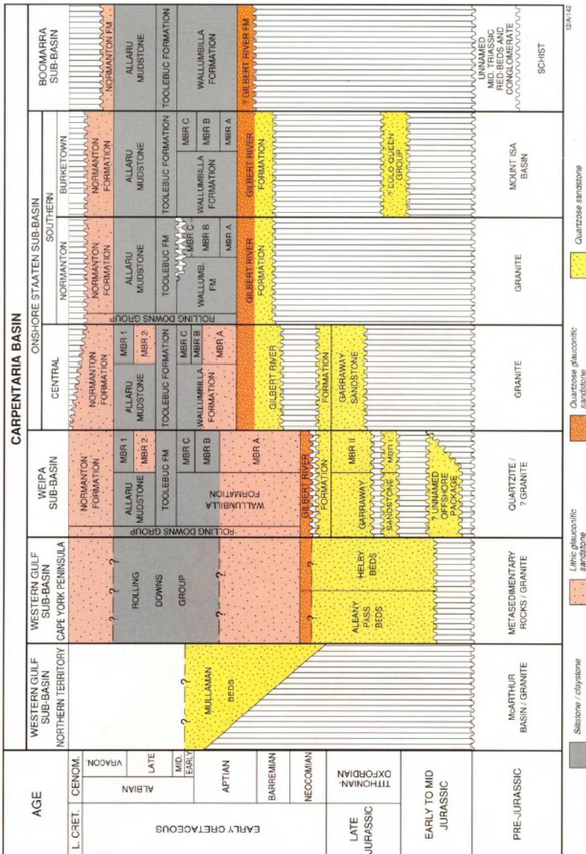
Figure 6: Lithostratigraphy, ages and correlations of the Carpentaria Basin(Draper, 1997)
