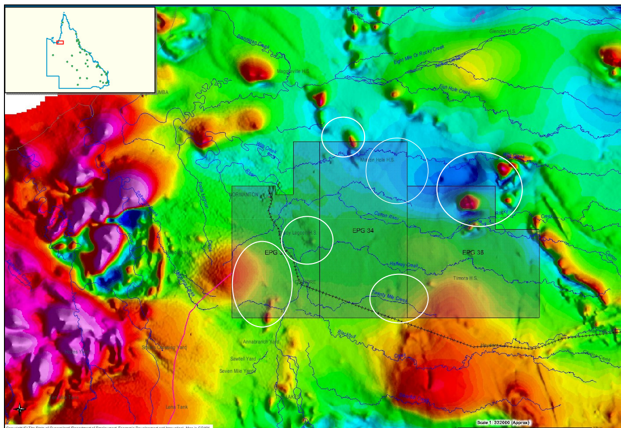
Figure 26: Prioritised targets on regional magnetic image TMI RTP
