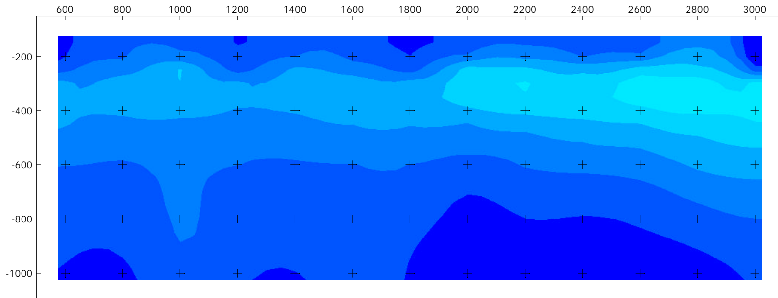
Line 5000 Emax Conductivity Depth Inversion mS/m Linear colour stretch 0 - 20
