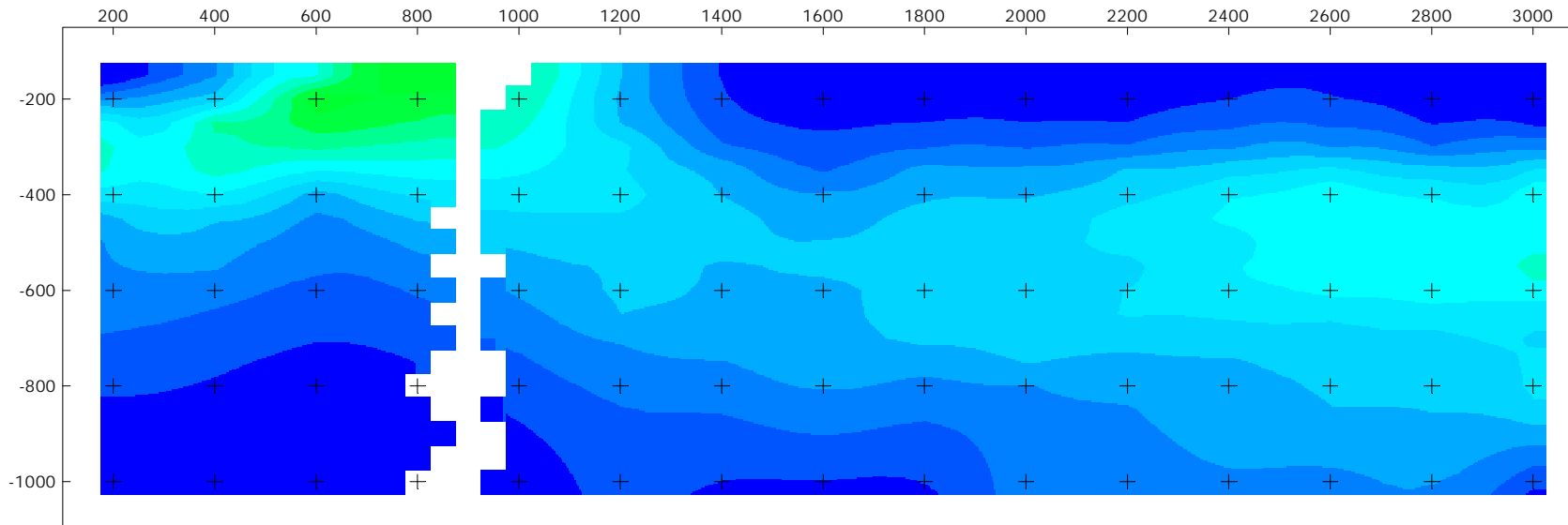
Line 2000 Emax Conductivity Depth Inversion mS/m Linear colour stretch 0 - 20
