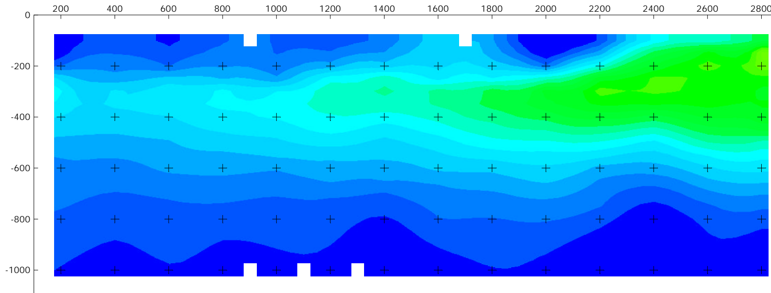
Line 3000 Emax Conductivity Depth Inversion mS/m Linear colour stretch 0 - 20
