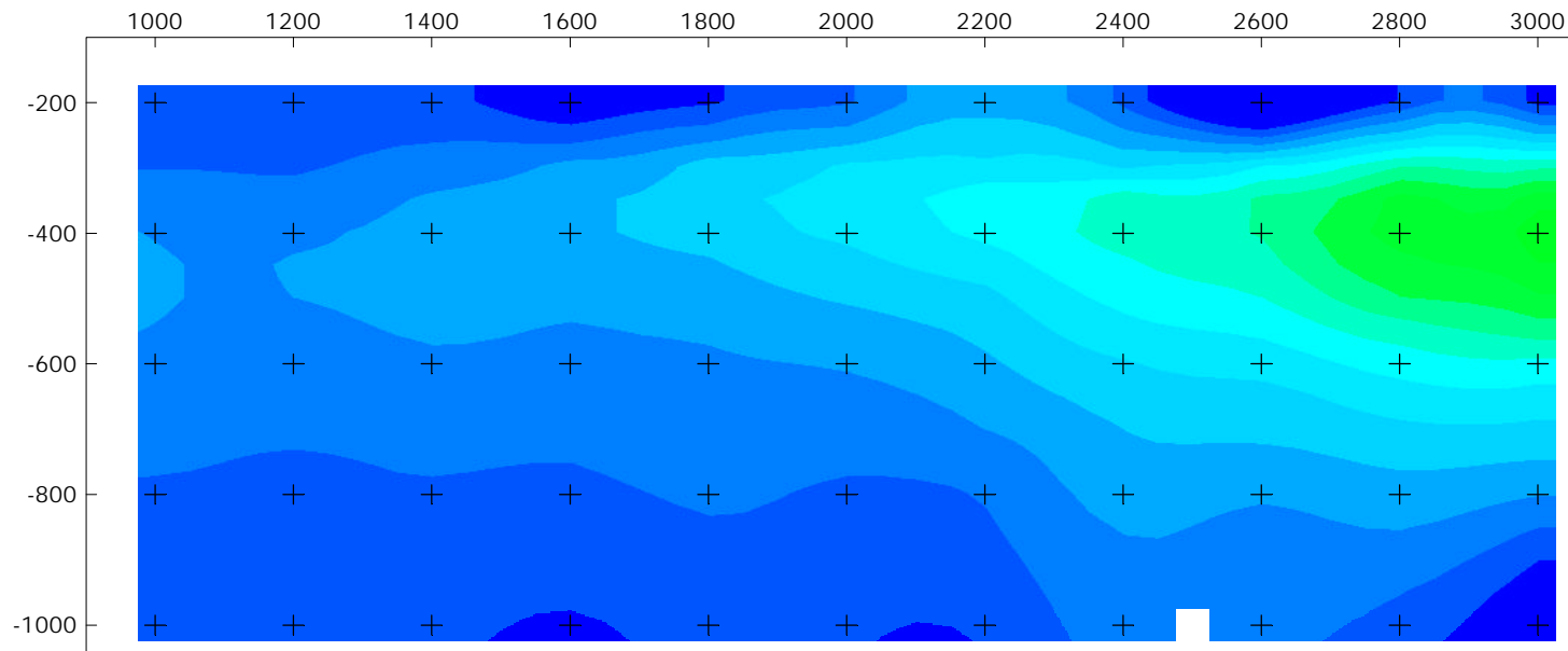
Line 4000 Emax Conductivity Depth Inversion mS/m Linear colour stretch 0 - 20
