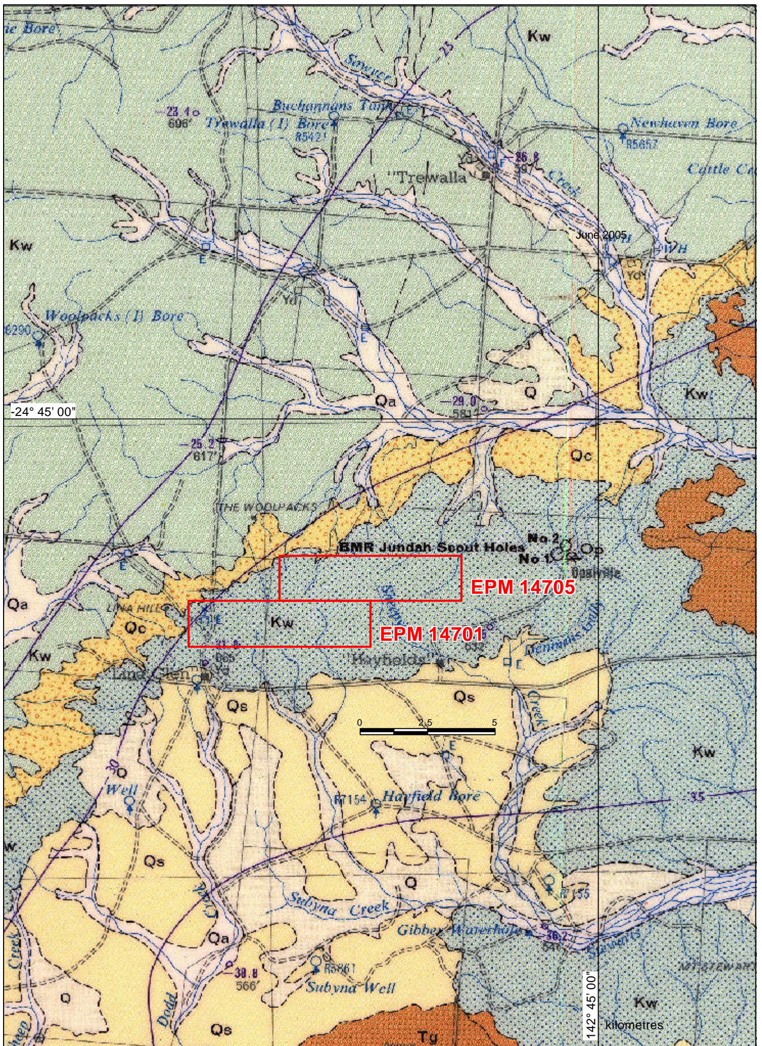
Figure 2: Geology of the Lina Glen Project
