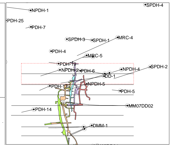
PLAN SCALE 1:2500
