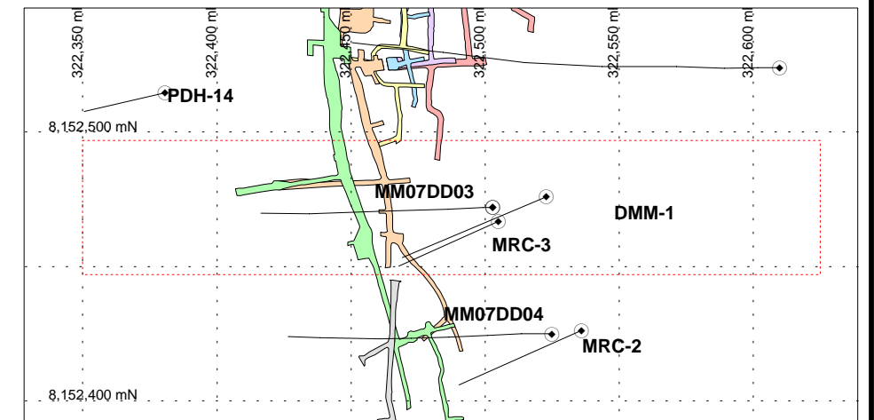
PLAN SCALE 1:2500
