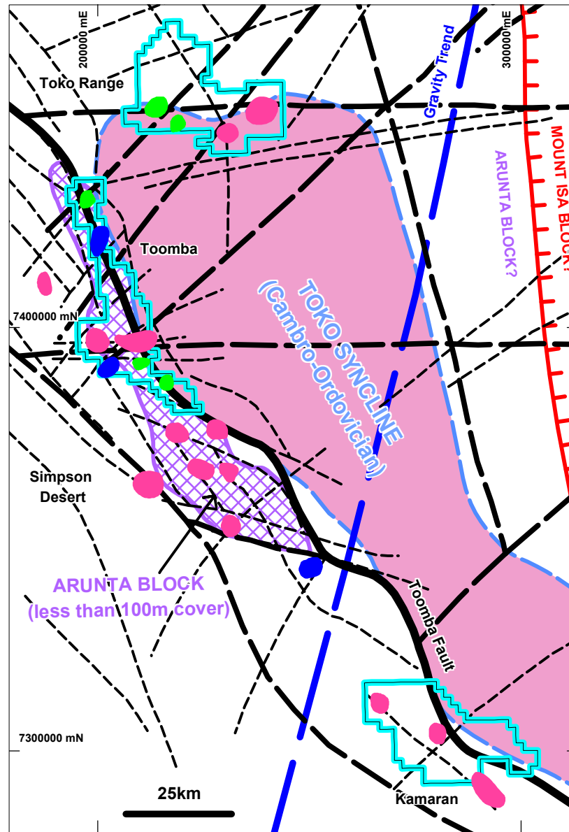
Toomba Fault Project - Major structures and geophysical features.
