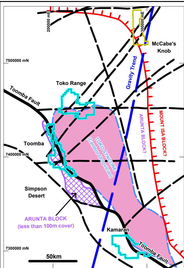
Toomba Fault Project - Interpreted major structures.
