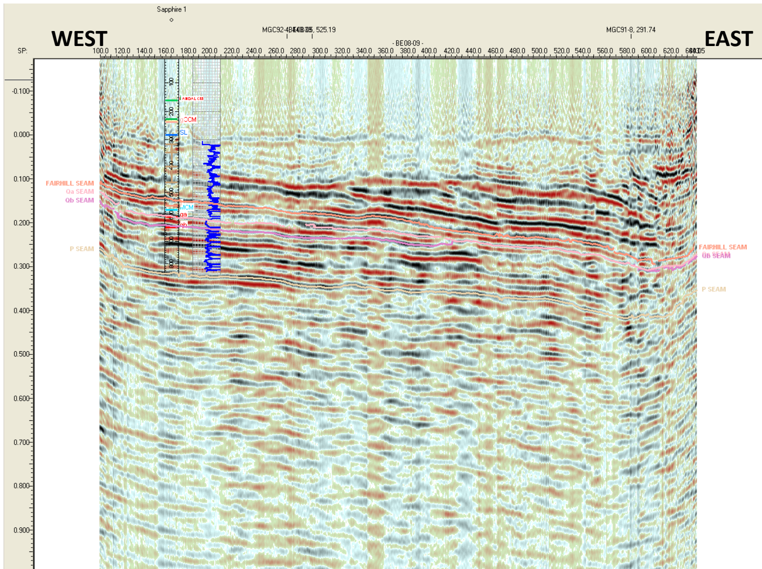
Line BE08-09
