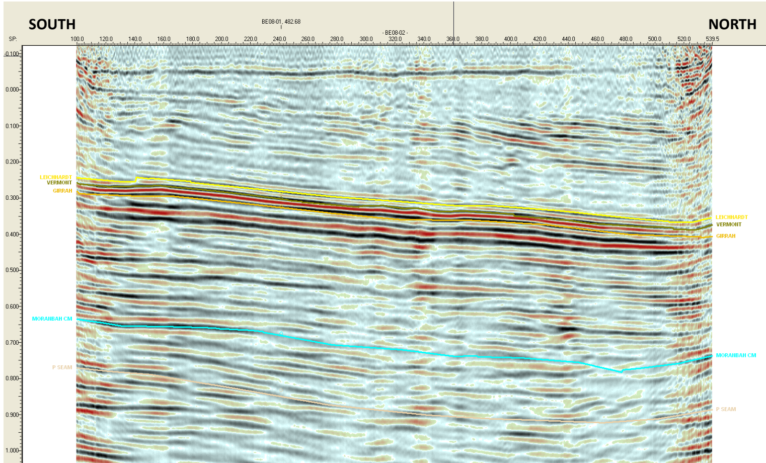
Line BE08-02
