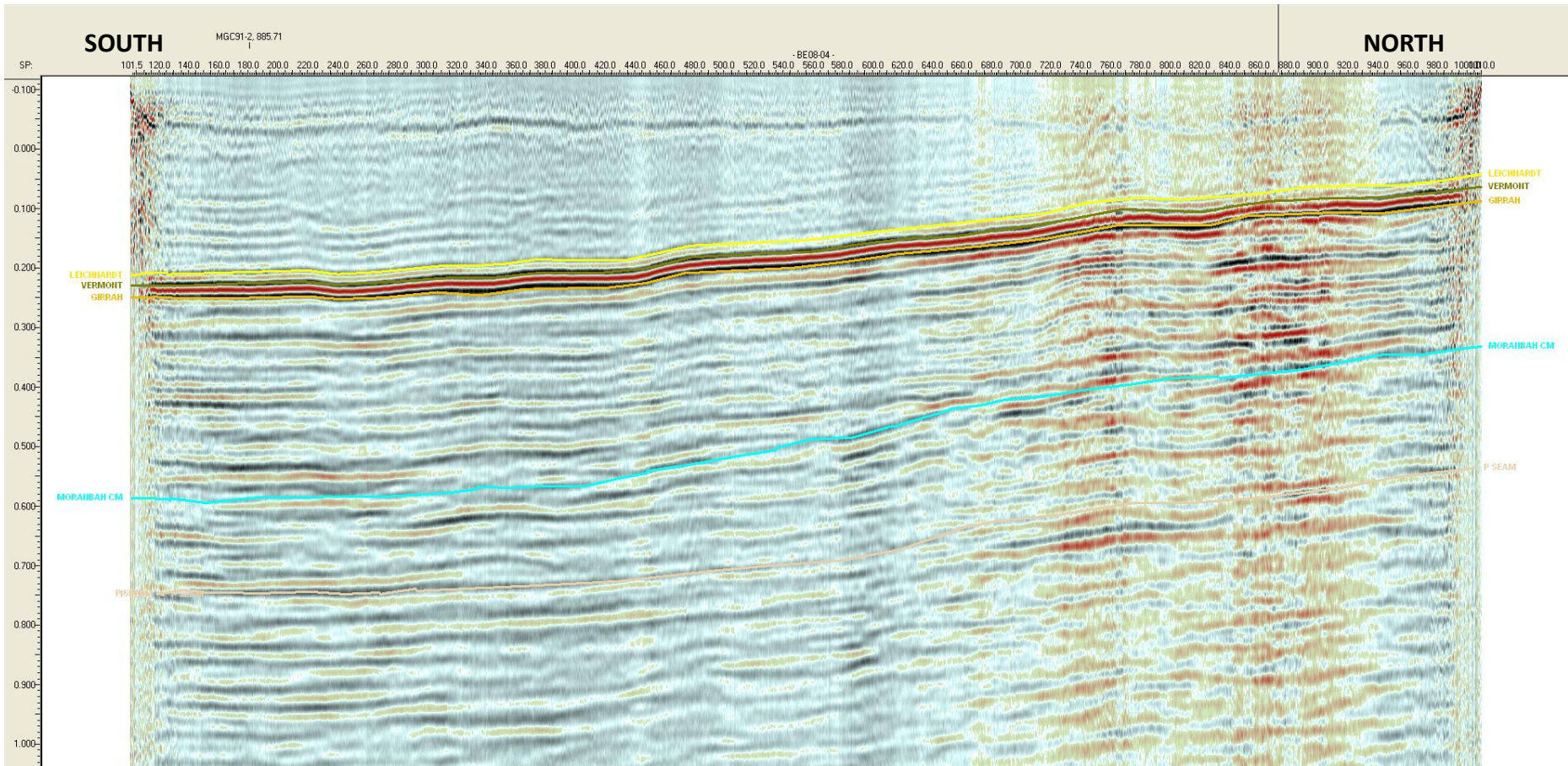
Line BE08-04
