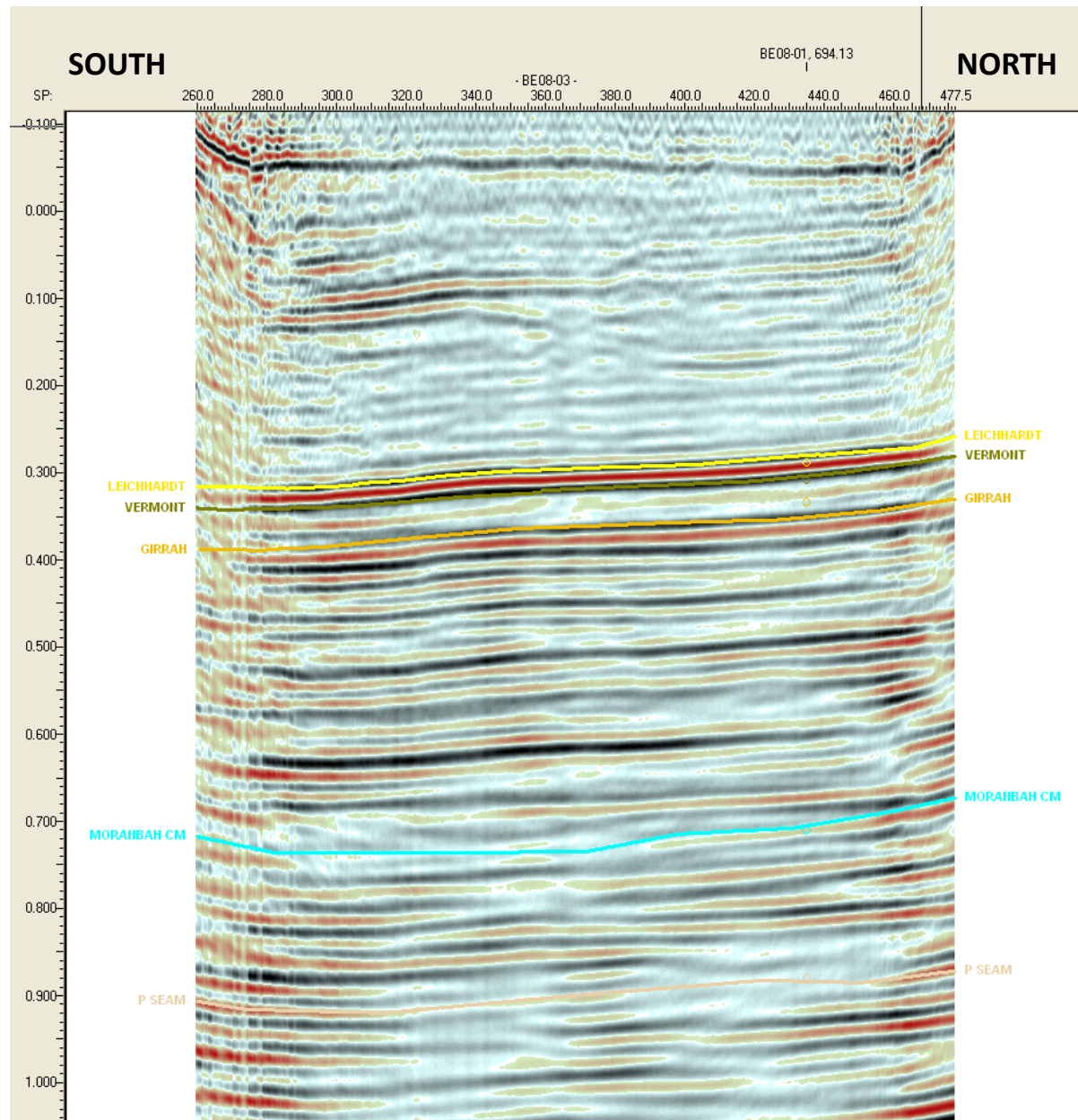
Line BE08-03
