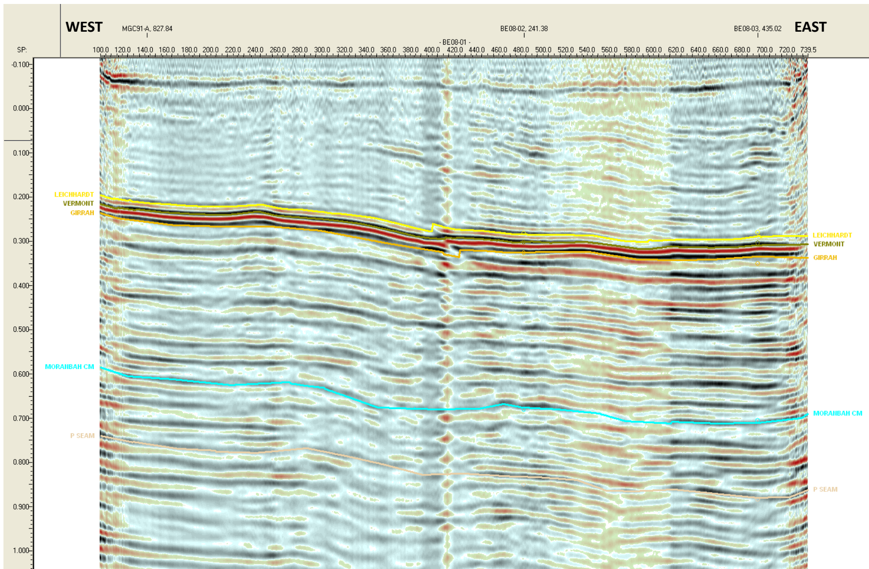
Line BE08-01
