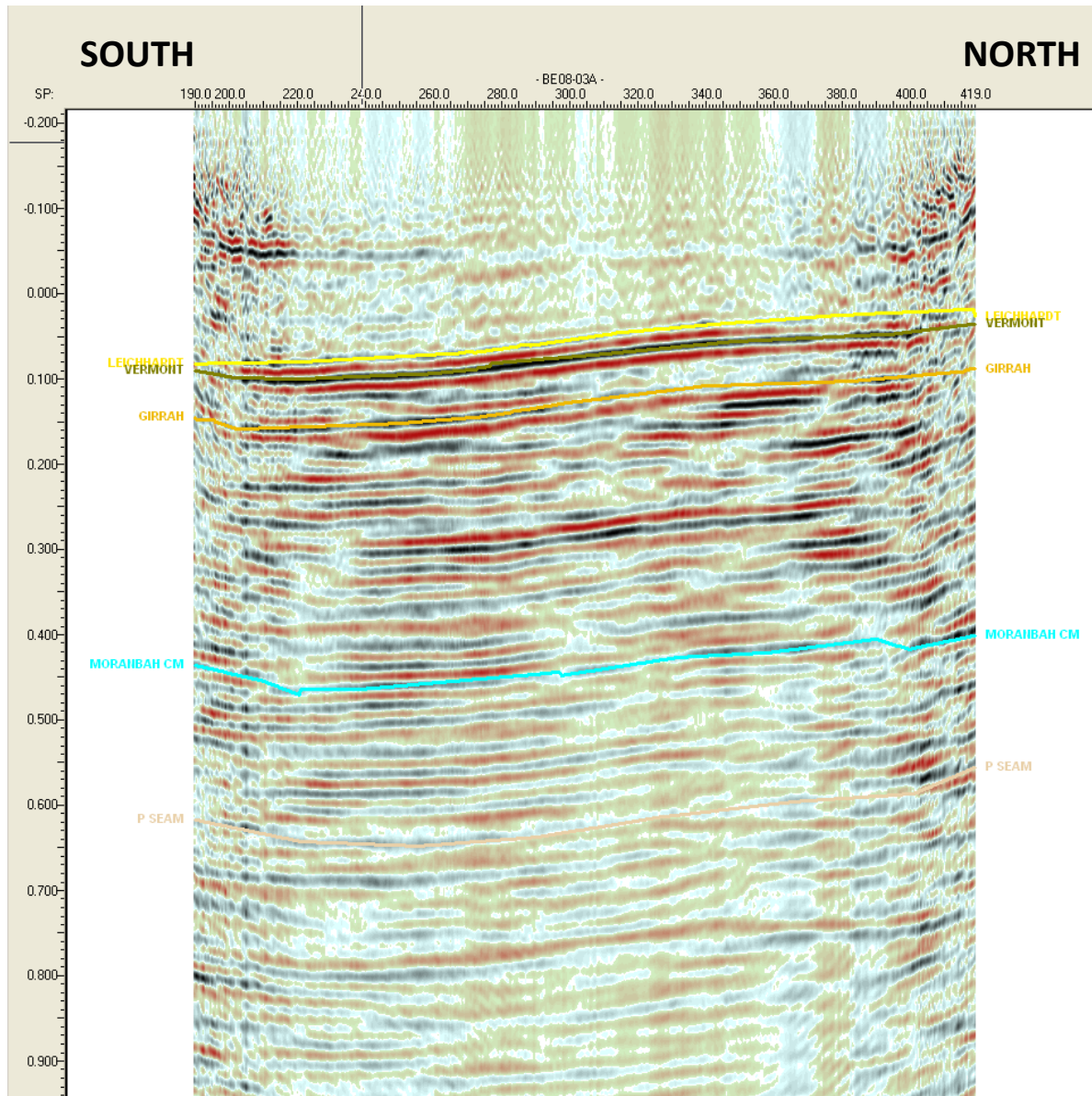
Line BE08-03A
