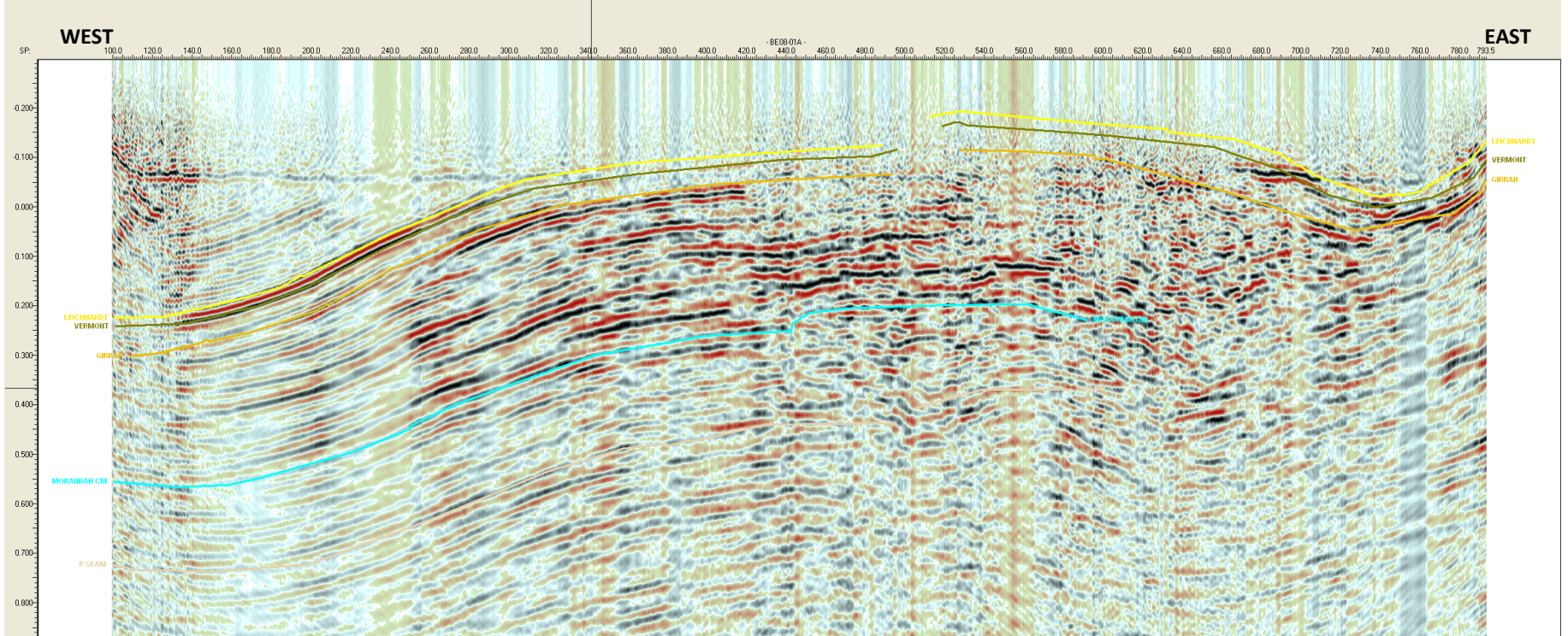
Line BE08-01A
