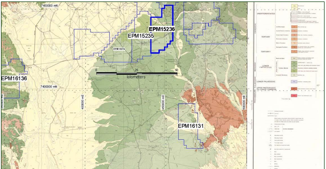
Figure 2: Geological map of the area of EPM15236
