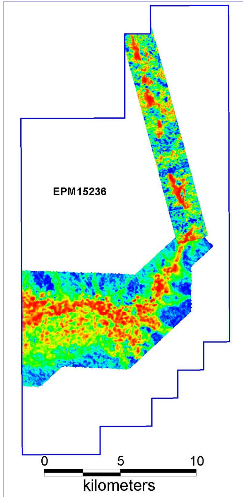
Figure 4: EPM15236 uranium channel from JV survey
