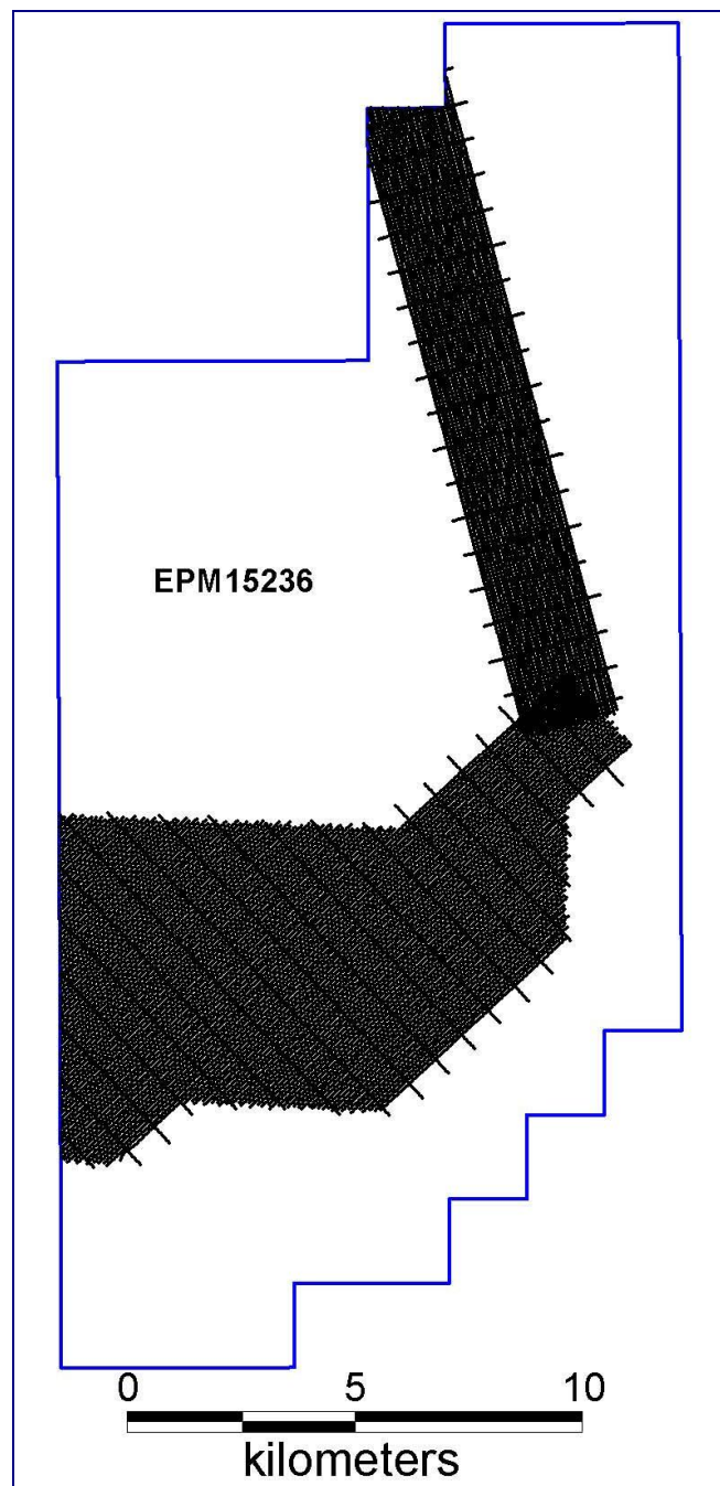
Figure 5: Radiometric survey flight lines EPM15236
