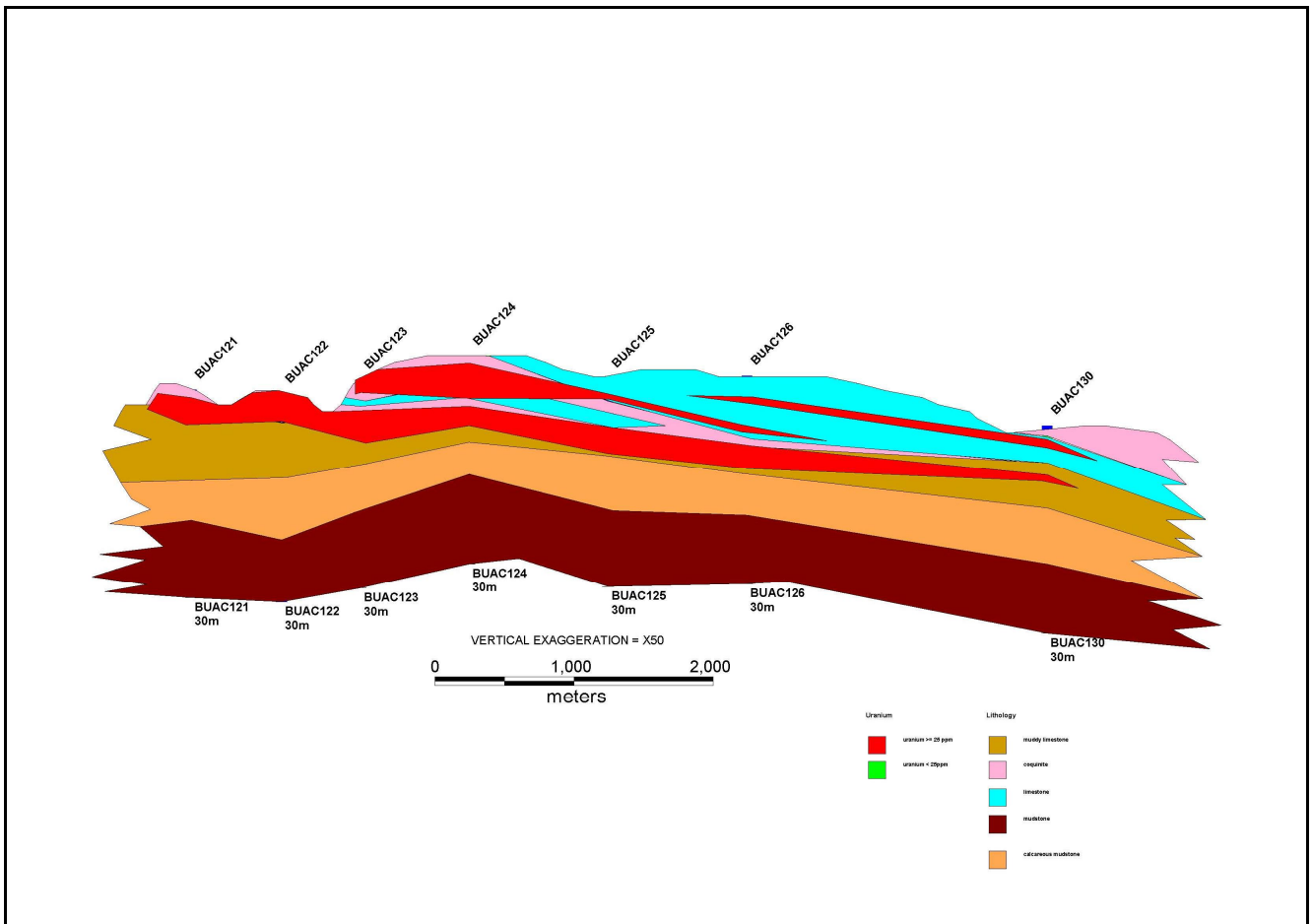
Figure 8: Interpreted NW-SE geological cross section - EPM15236
