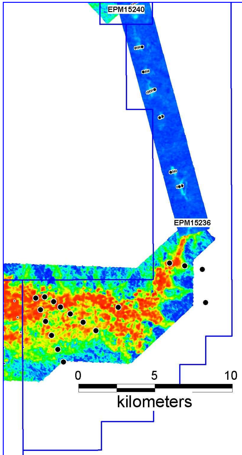
Figure 6: Location of air core drill holes in EPM15236 (uranium radiometric image)
