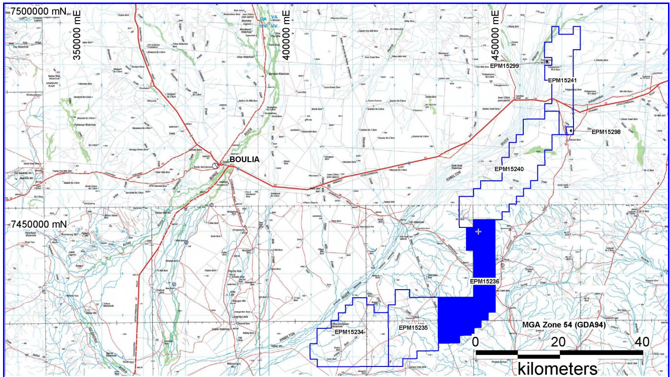
Figure 1: Location map EPM15236
