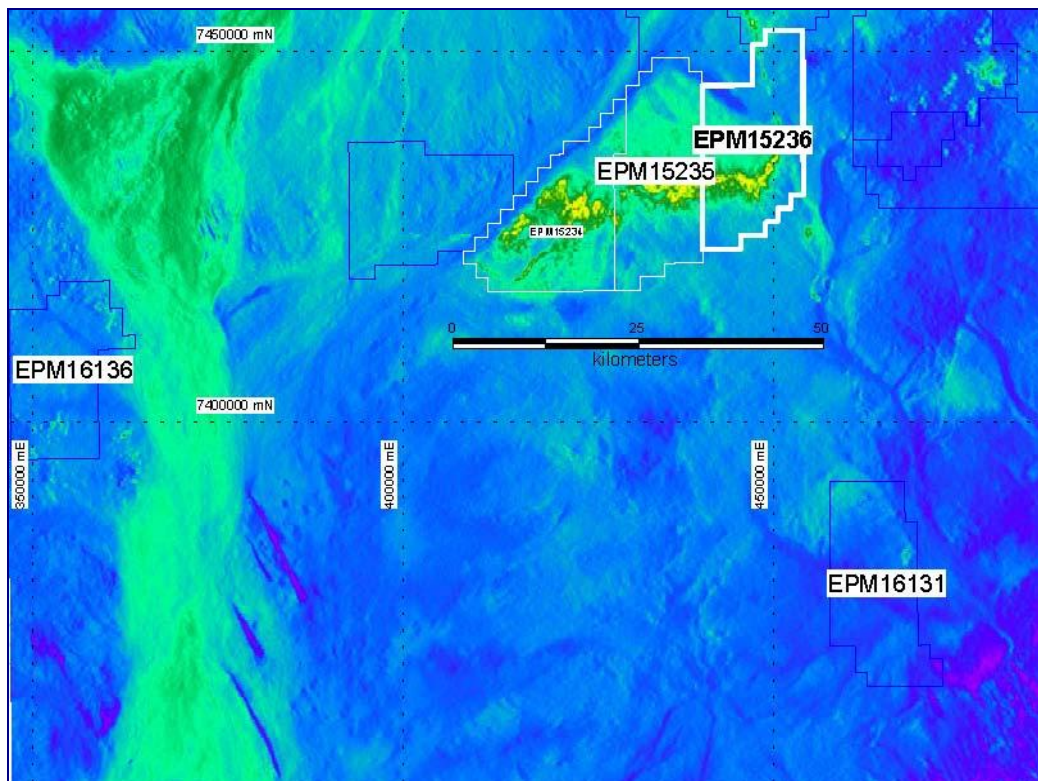
Figure 3: Total count radiometrics from DME regional survey
